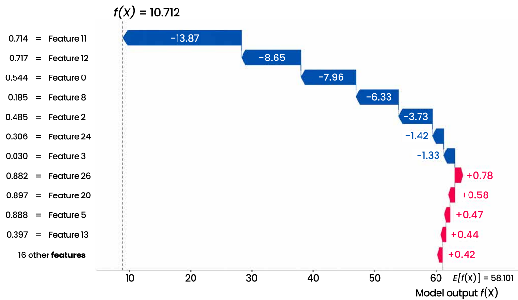
Fig. (9). Local SHAP explanation for a held-out measurement state.
