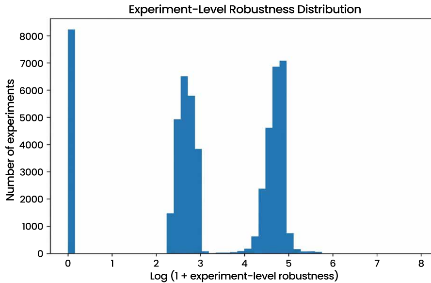
Fig. (15). Experiment-level distribution of the released robustness target.
