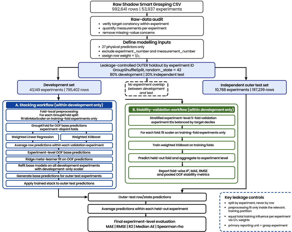
Fig. (1). Leakage-controlled outer holdout, stacking and stability-validation workflow.
