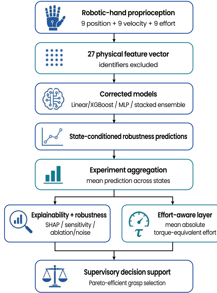
Fig. (4). Validated retrospective framework for experiment-level robustness prediction and post-episode effort-aware assessment.
