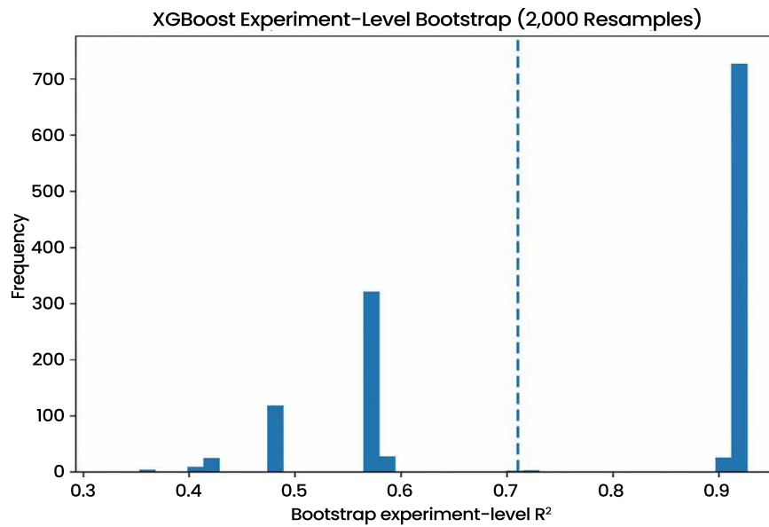
Fig. (3). Experiment-level bootstrap distribution of R^2 (2,000 Resamples).
