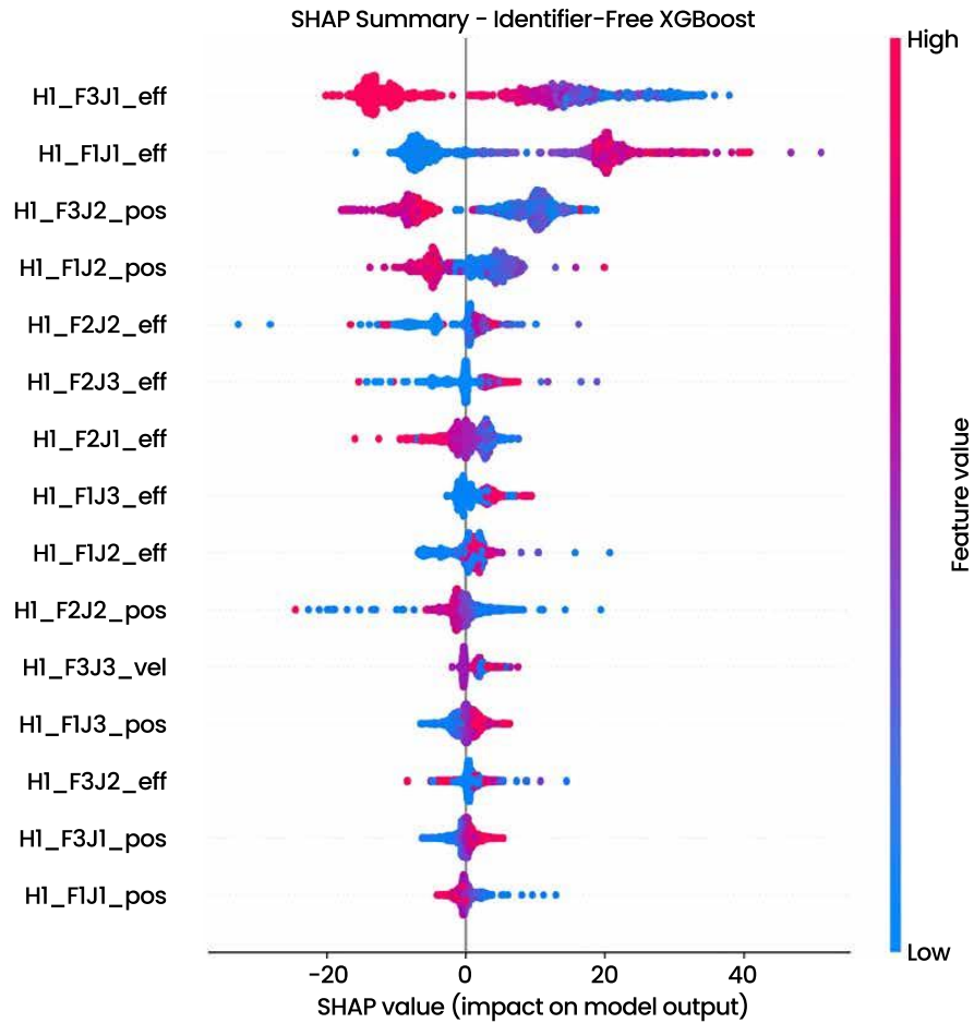
Fig. (8). SHAP summary plot for the 27-channel XGBoost model.
