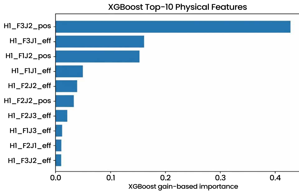
Fig. (6). XGBoost Top-10 feature importance (Identifiers Excluded).
