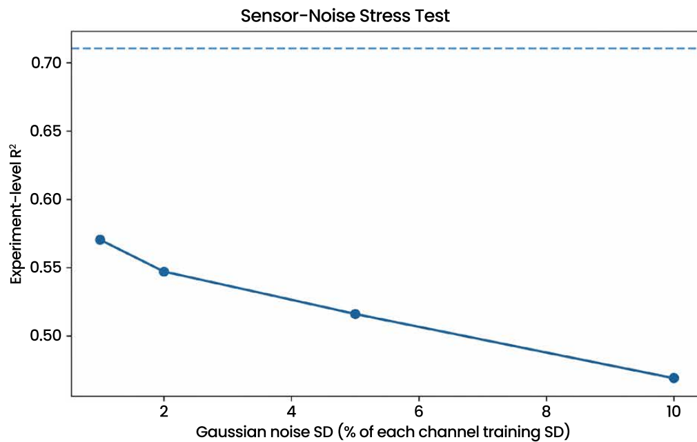
Fig. (18). Synthetic noise stress test of model predictions (not hardware sensor validation).
