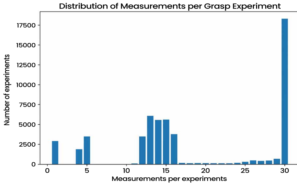
Fig. (12). Distribution of measurement counts per grasp experiment.
