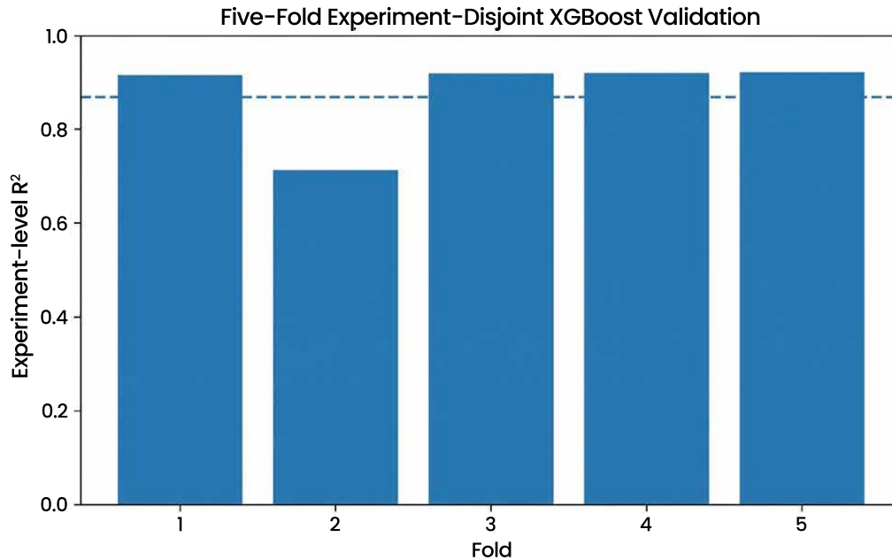
Fig. (16). Five-fold experiment-level XGBoost R^2 .
