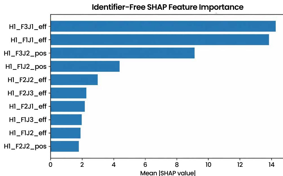
Fig. (7). Global SHAP importance for the identifier-free XGBoost model.
