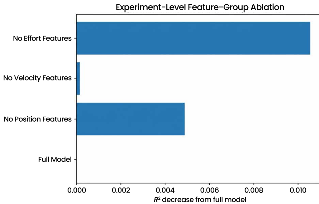
Fig. (17). Experiment-level feature-group ablation.
