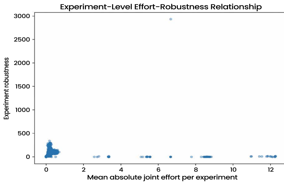
Fig. (13). Retrospective experiment-level mean absolute actuation effort versus grasp robustness.
