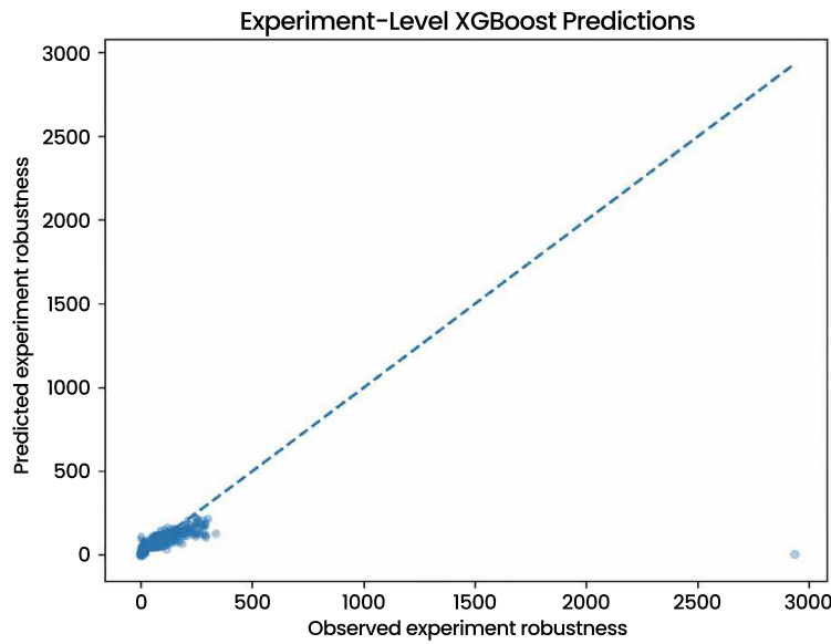
Fig. (10). XGBoost: experiment-level actual versus predicted robustness.
