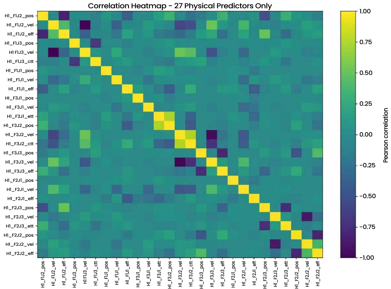
Fig. (2). Identifier-free correlation heatmap of the 27 physical proprioceptive variables.
